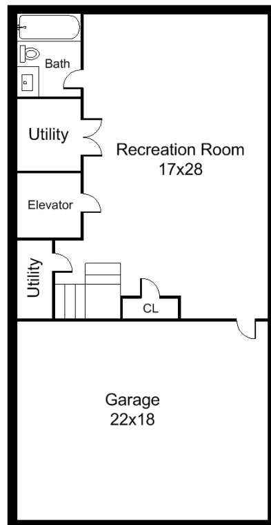
Ground Floor / Basement
