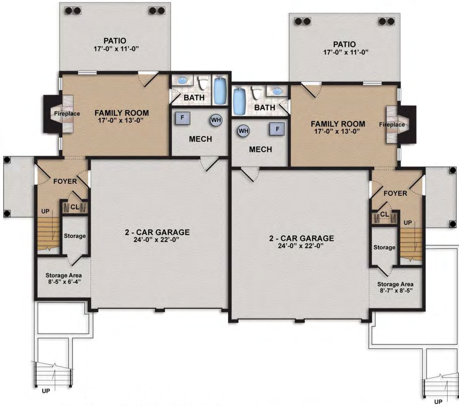
LOWER LEVEL FLOOR PLAN UNIT A
